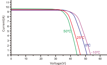
I-V characteristics at different temperatures (AM1.5, 1000W/m 2 )
